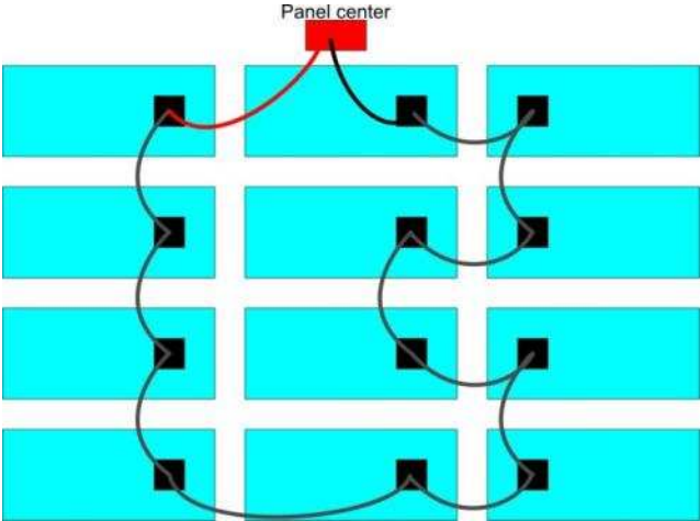
How the panels were connected in series to allow for a minimum use of transfer cable.
