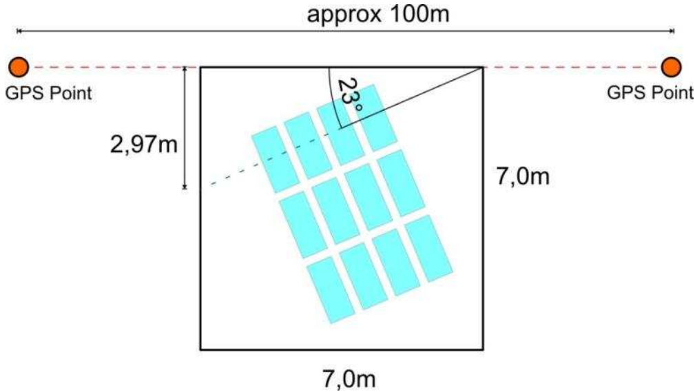
Illustration showing how the solar panels were aligned to become properly oriented to the east.
