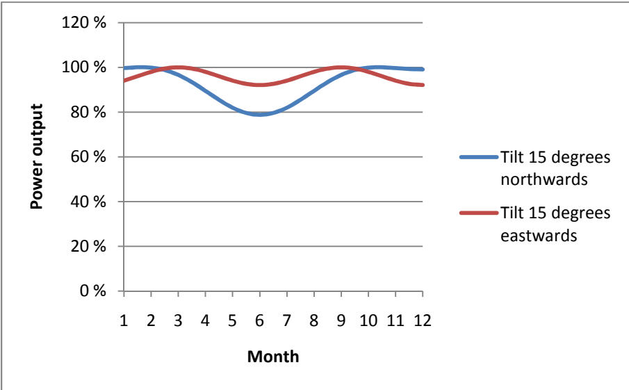
Diagram showing that the seasonal fluctuations in power output are bigger when the panels are tilted northwards, which would be the traditional orientation.
